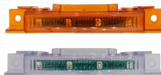
FLTCBV65004A FLTCBV65004AC 4 LED | 7.5-14 VDC
